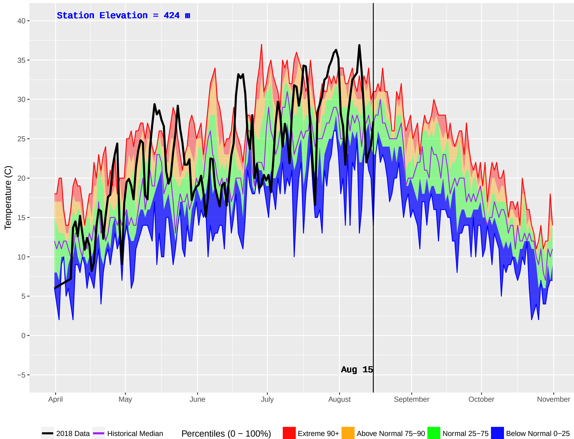
SPLINTLUM (1055) : Historical (2009–2016) and Current (2018) Daily Temperature
