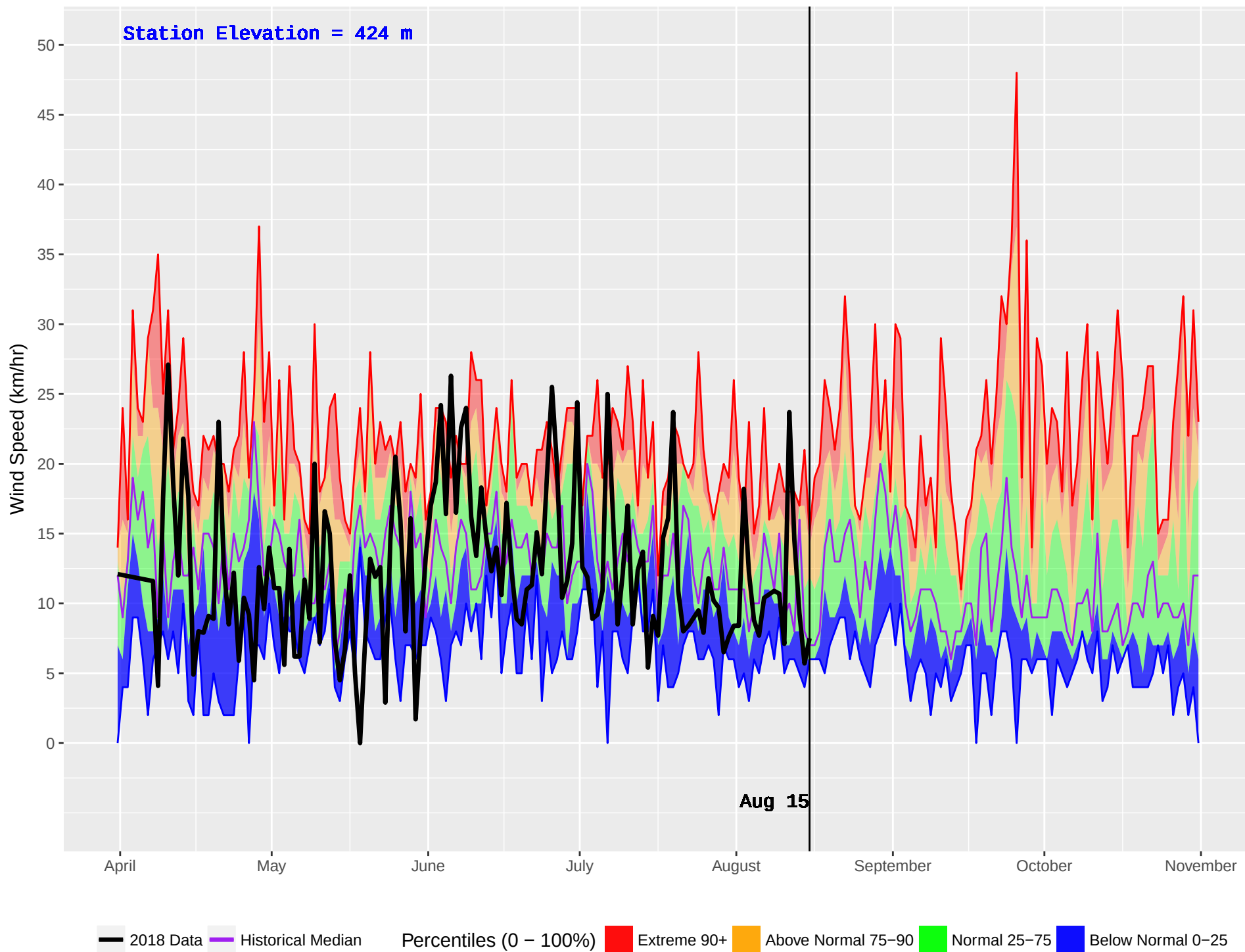
SPLINTLUM (1055) : Historical (2009–2016) and Current (2018) Daily Wind Speed
