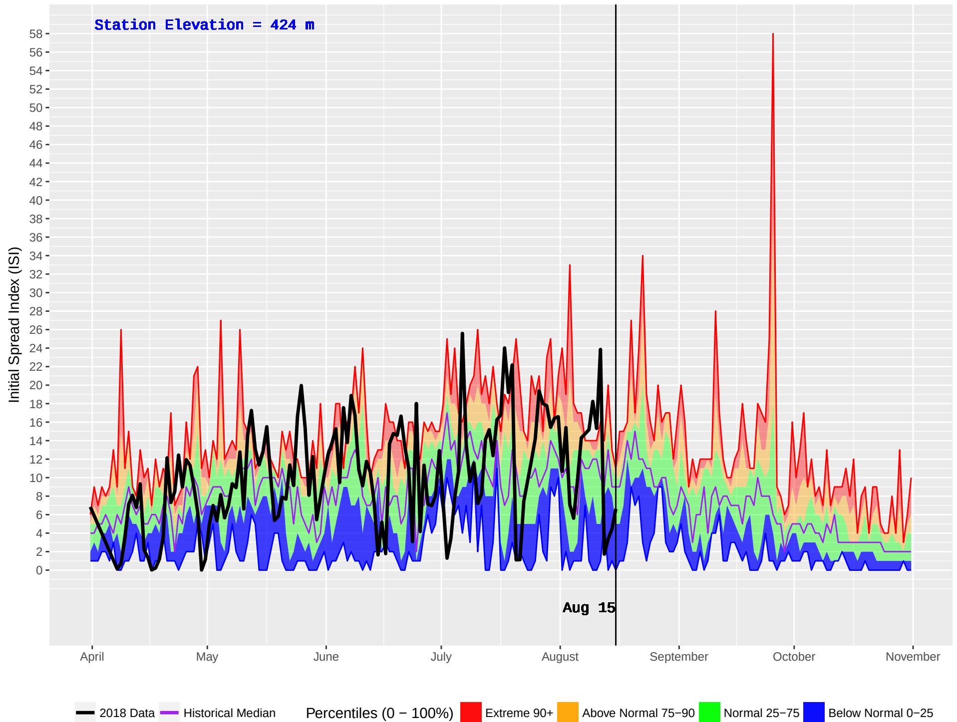
SPLINTLUM (1055) : Historical (2009–2016) and Current (2018) Daily Initial Spread Index (ISI)
